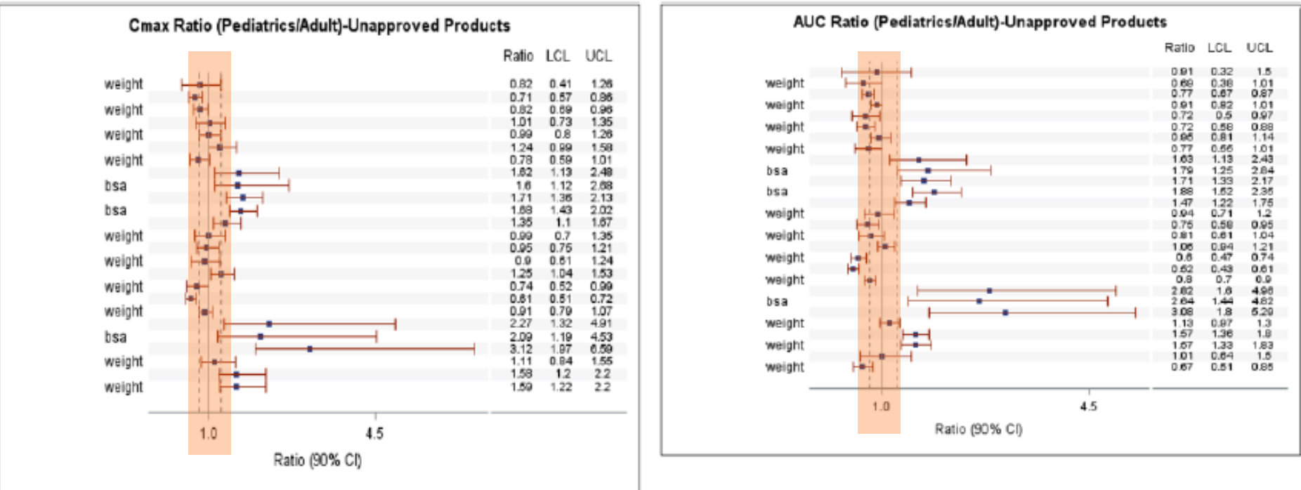
Figure 3. Forest plot of C_{max} and AUC ratios (pediatric/adult) for products without a pediatric indication. The solid line corresponds to a ratio of 1. The 90% confidence intervals are based on the Fieller method.
